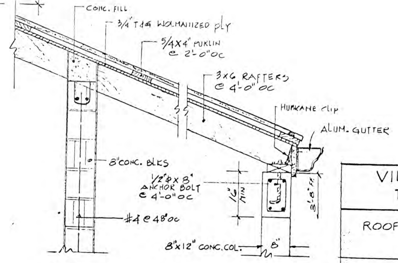
B SECTION 1" = 1'-0"
