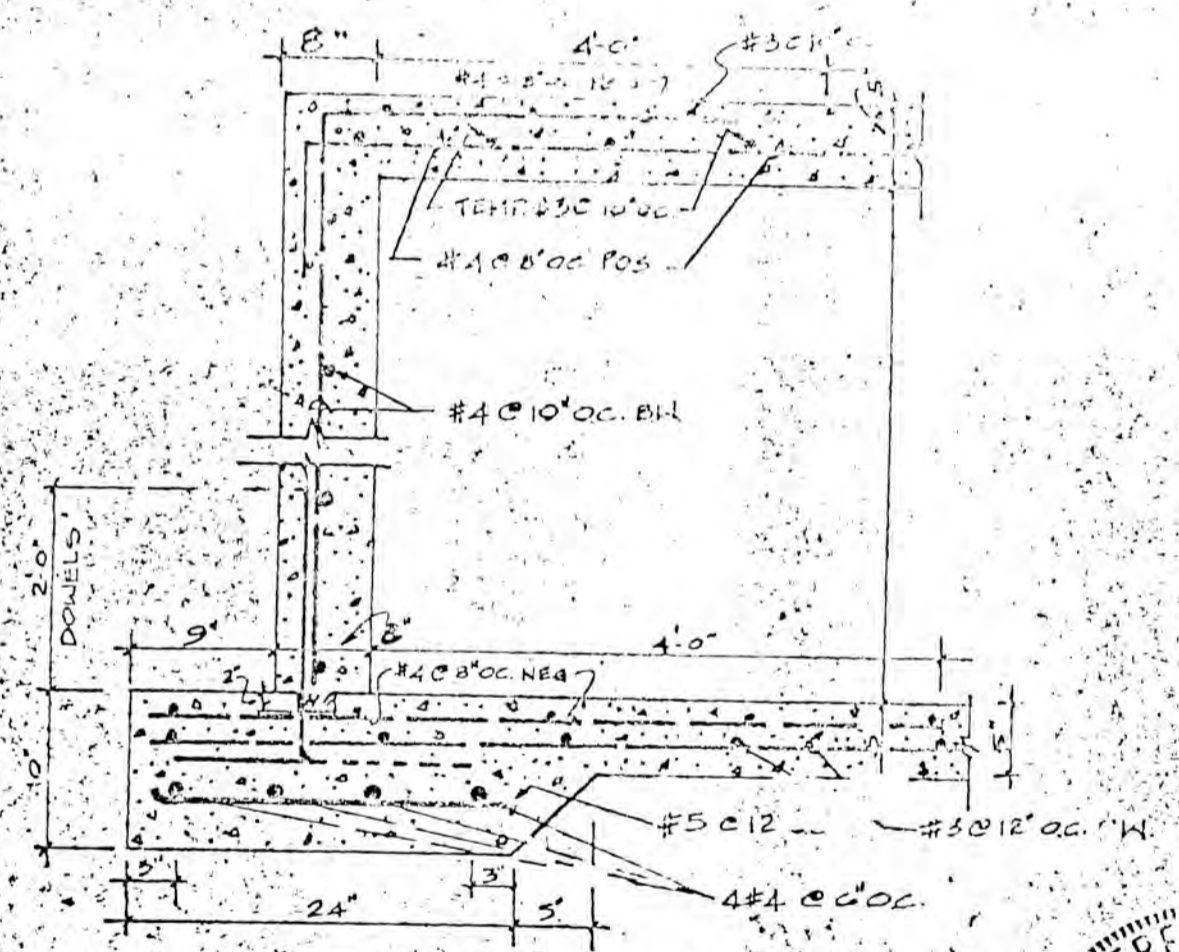
CISTERN DETAIL F-2
