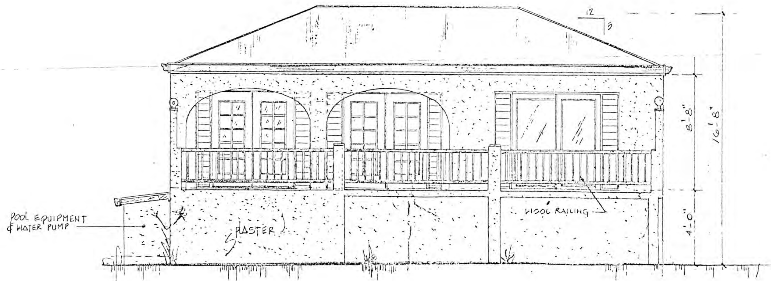
NORTH ELEVATION
