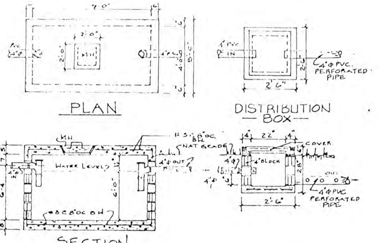
SEPTIC TANKS DETAILS
