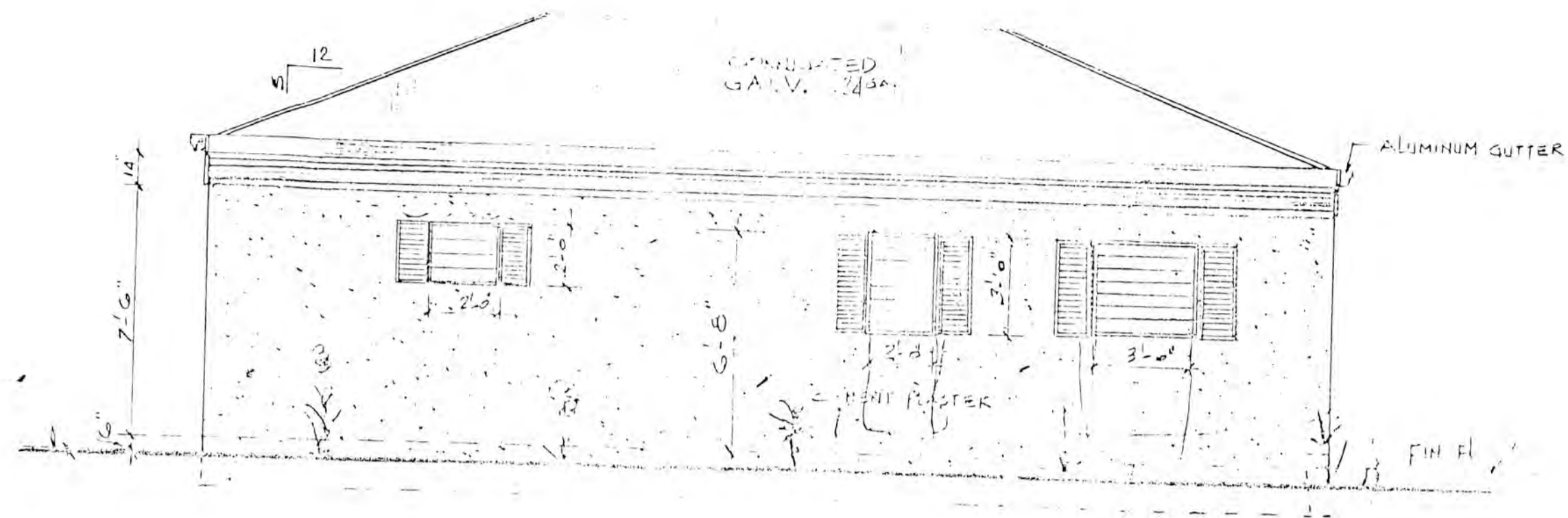
SOUTH ELEVATION SC 1/4"=1'-0"
