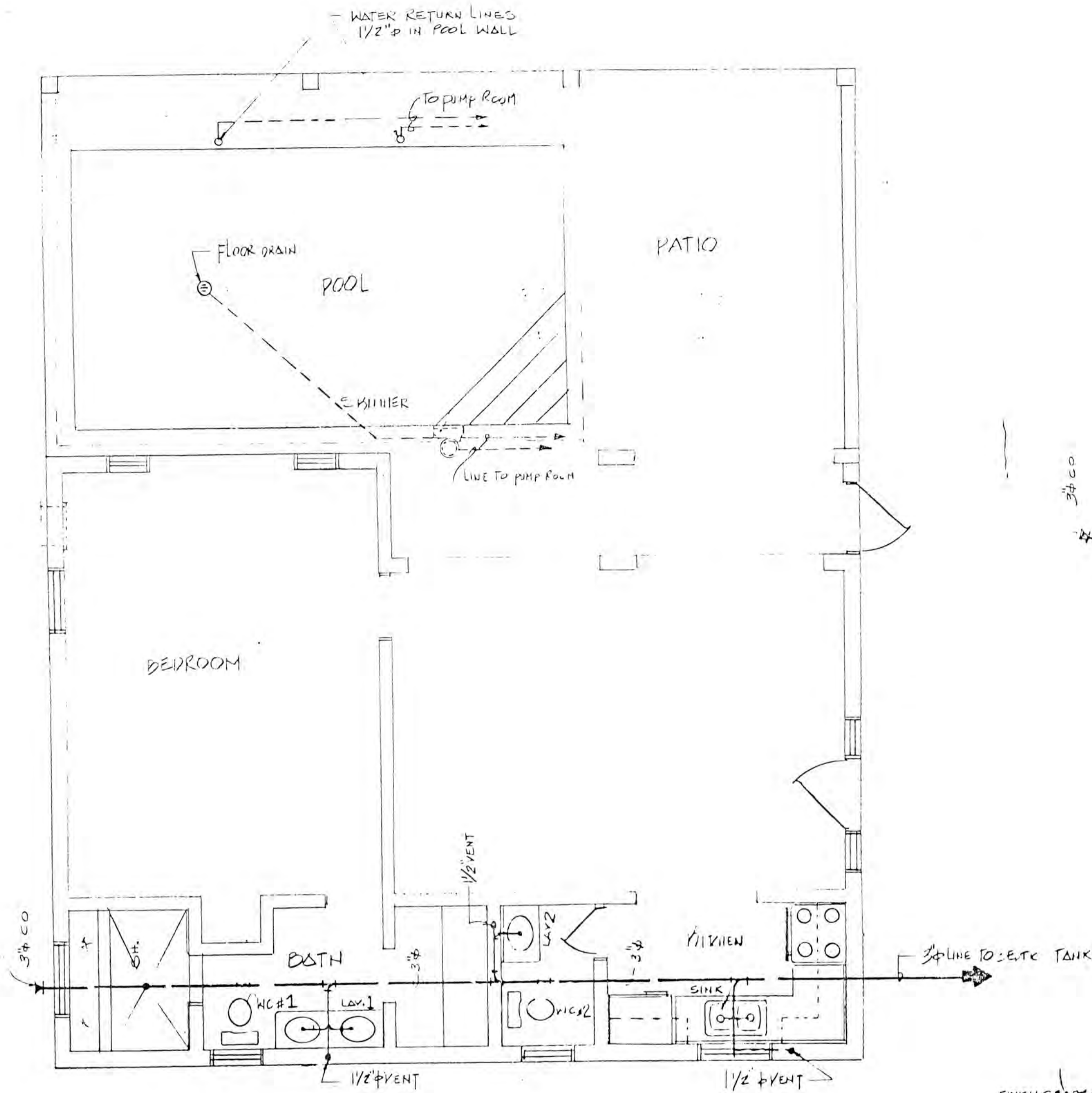
PLUMBING PLAN
