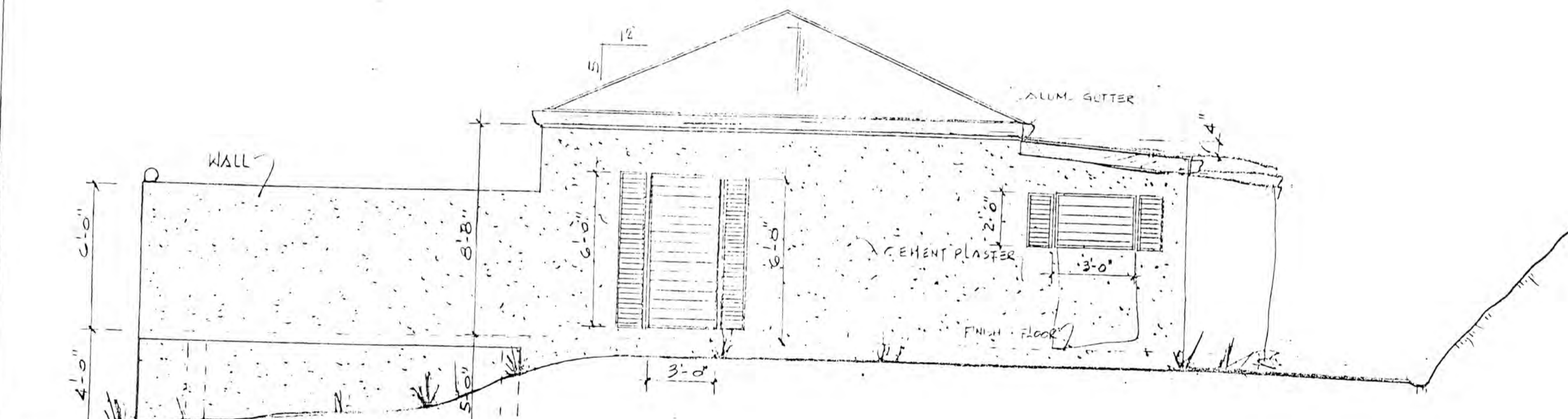
WEST ELEVATION SC 1/4"=1'-0"
