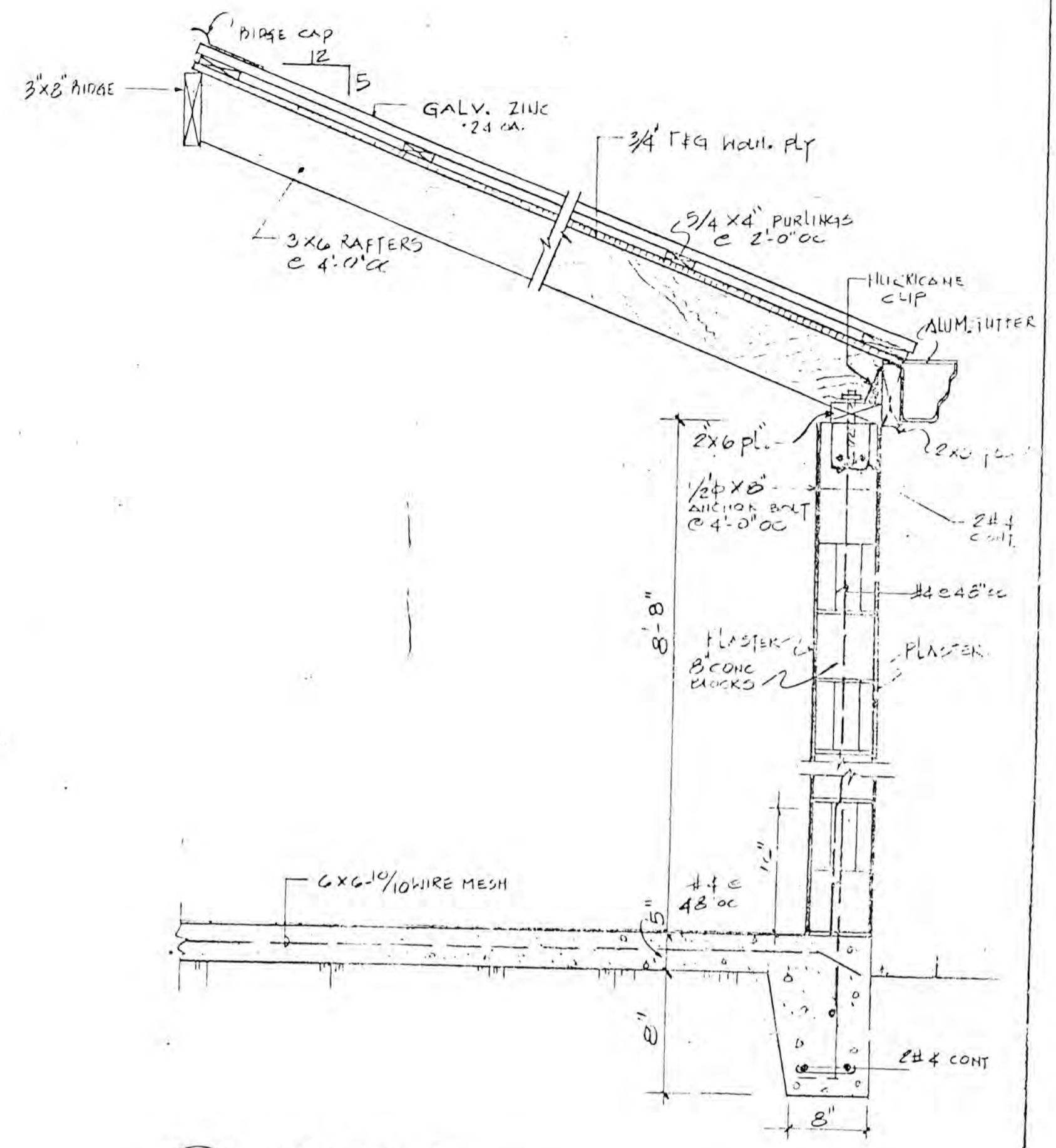
A SECTION 1" = 1'-0"
